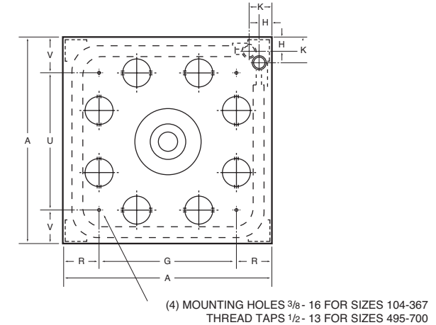
Figure 4 - Sizes 104-700
