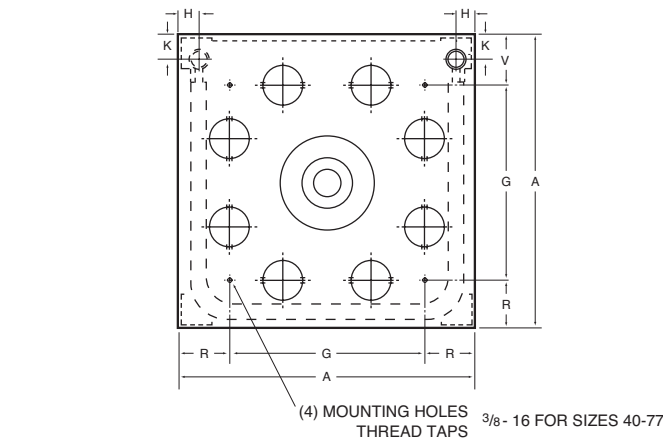
Figure 3 - Sizes 40-77
